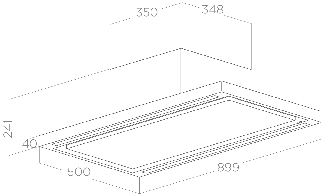
FALSE CEILING CUT: 480X880
