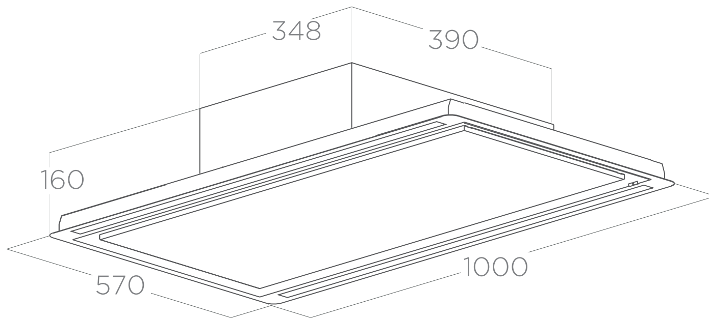
FALSE CEILING CUT: 550X980
